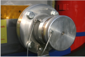
Bottom fill dry break couplers for diesel/petrol and aviation fuels
