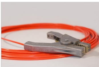
Earth cable and approved clamp for aviation fuelling and petrol transfer
